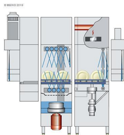
Schematic sectional view of machine
