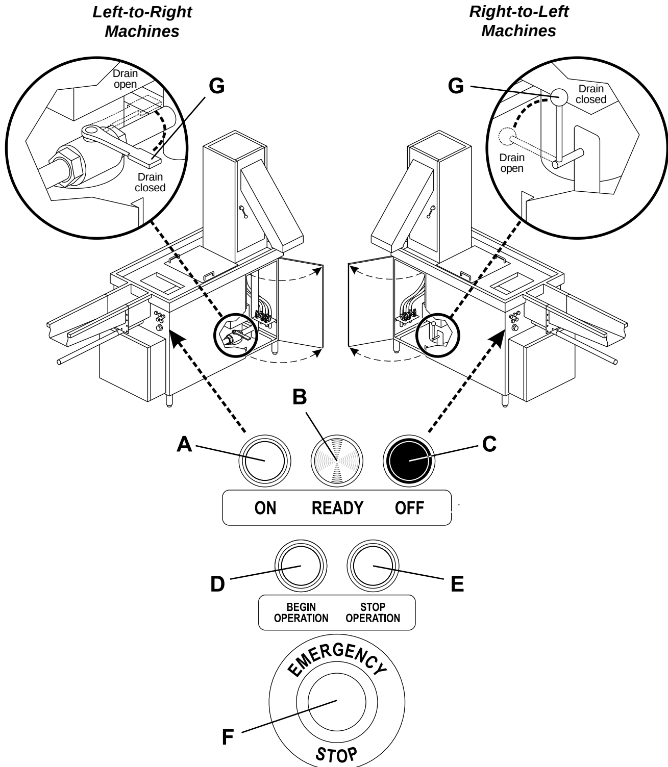
Figure 4-1: Waste pulper controls
