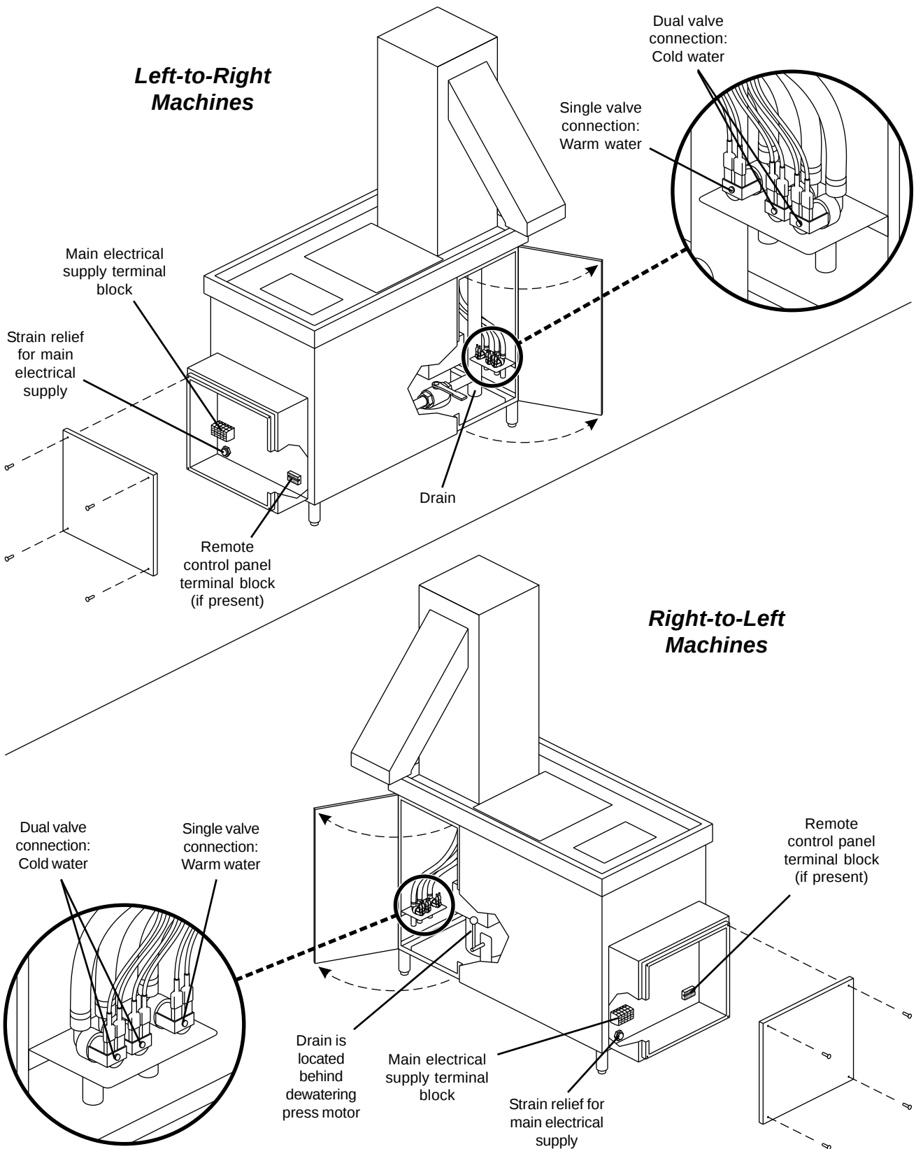
Figure 3-3: Utility connections
